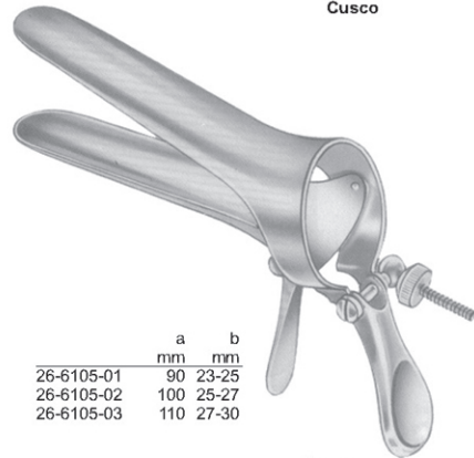
Cusco Swiss Pattern
