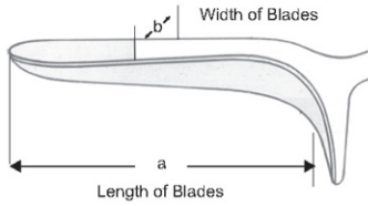
Scheme of Dimensions for Specula
